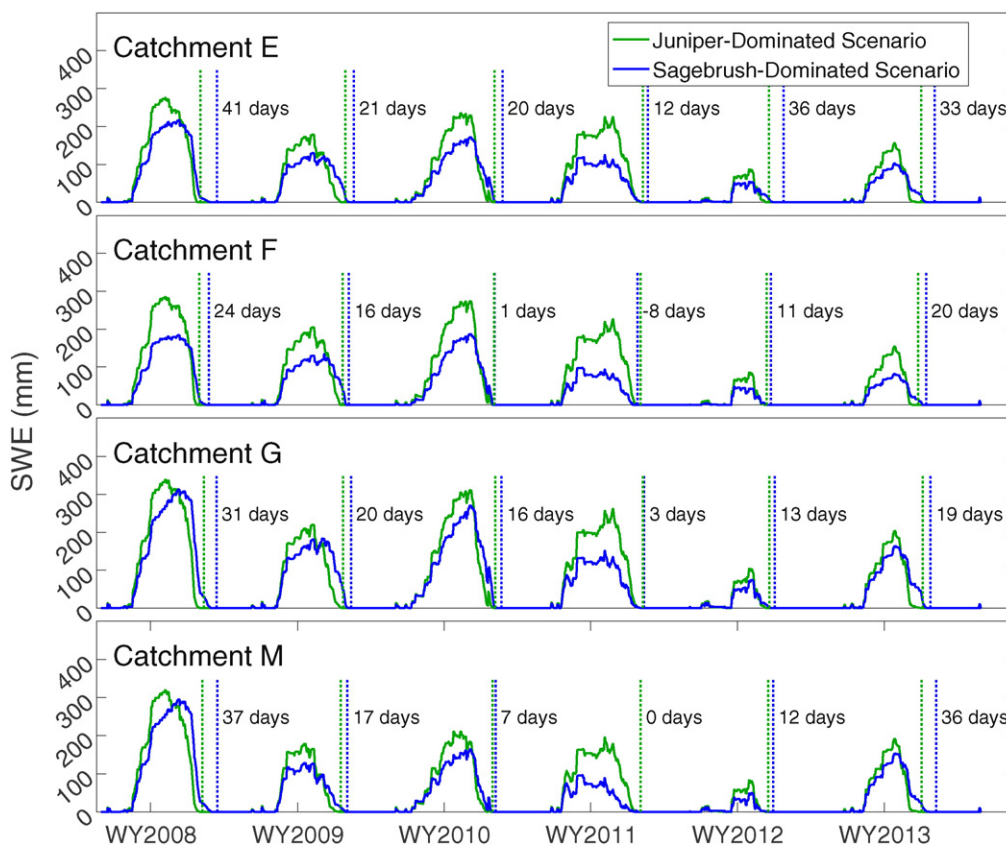
Figure 6. Modeled mean basin snow water equivalent (SWE) for juniper- and sagebrush-dominated scenarios showing higher peak accumulation and earlier melt out for juniper-dominated scenario in number of days.
