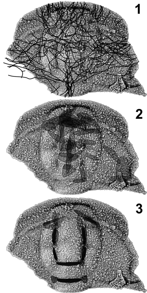
Figure 20. Composite maps showing effect of taphonomic compaction on crania of Oryctocephalites palmeri preserved in shale ( n = 28 ). (1) Locations of fractures. (2) Sites of cranial distortion. (3) Sites of increased furrow depth. Darker shaded areas in (2) and (3) indicate overlap between specimens.
