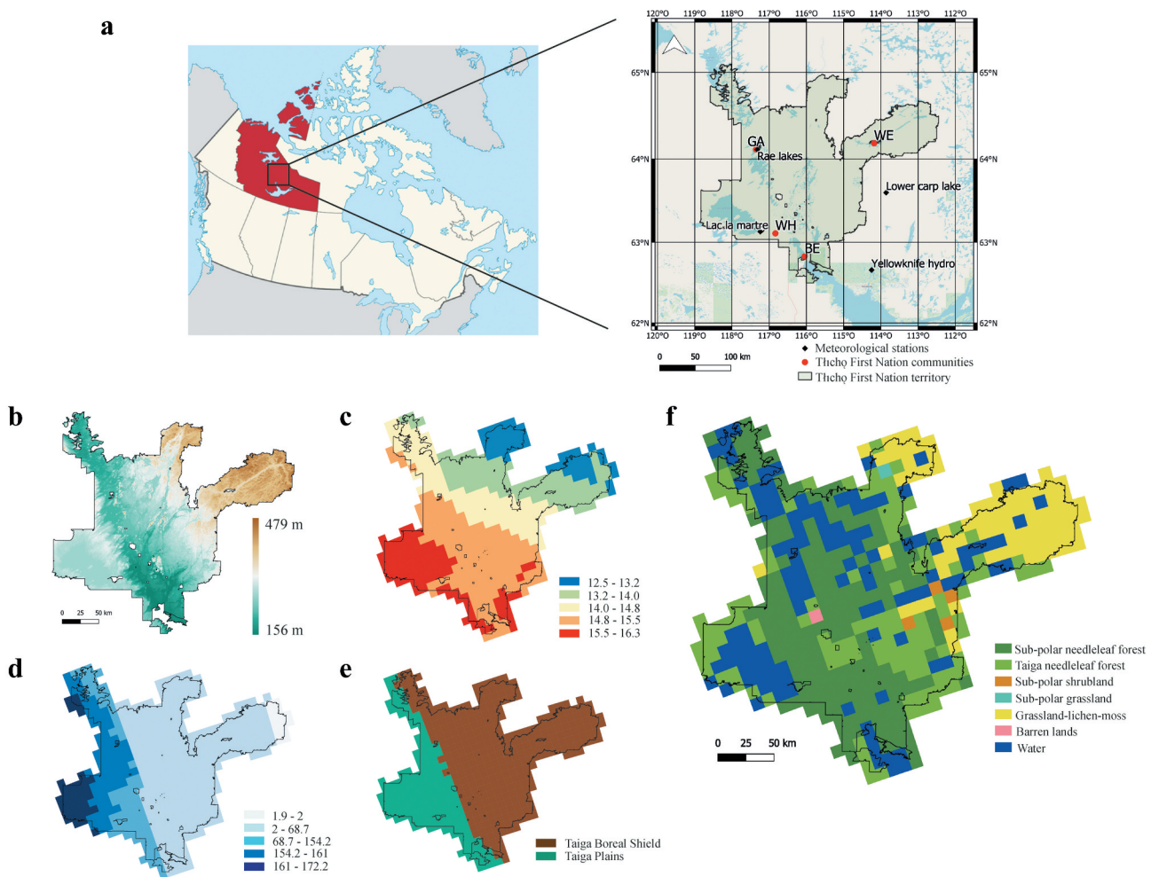
Figure 1. (A) Location of the study area encompassing the four communities of the Tẖcẖo First Nation in the Northwest Territories, Canada (GA = Gamètì, WH = Whatì, BE = Behchokò, WE = Wekweètì). (B) Elevation at 10-m spatial resolution (in meters). (C) 1965–2019 mean temperature gradient (southwest to northeast) at noon (degrees Celsius) for the fire season period extracted from four weather stations and interpolated with BioSIM in 10-km grid cells and (D) 1965–2019 sum of precipitation (mm) gradient (northeast to southwest) for the fire season period interpolated with BioSIM. (E) Soil-based ecoregion classification in 10-km grid cells. (F) Main land cover types in 2010 per 10-km grid cell.
