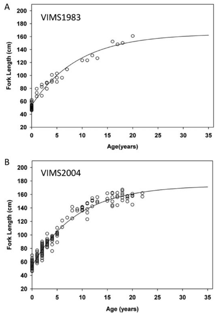
FIGURE 4. VB3 model fits and length-at-age data for male Sandbar Sharks from the (A) VIMS1983 and (B) VIMS2004 data sets.
