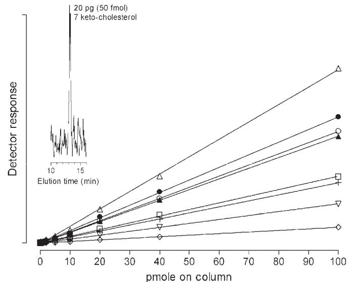
FIG. 3. (Oxy)sterols produce linear calibration curves over a broad dynamic range. Differences in sensitivity result from differences in ionization and fragmentation efficiencies. From top to bottom: 7 \beta -hydroxycholesterol; cholestane-3,5,6-triol; 5,6 \alpha -epoxycholesterol; 25-hydroxycholesterol; 7-ketocholesterol; desmosterol; and 5,6 \beta -epoxycholesterol and cholesterol. The inset shows the signal:noise ratio at the lower level of detection of 7-ketocholesterol.
