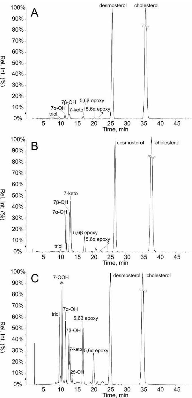
FIG. 4. Detection of (oxy)sterols in Percoll-washed sperm cells by MRM-MS. A ) Bovine sperm cells directly after ejaculation. B ) Sperm cells incubated in the presence of oxidants. C ) Small unilamellar vesicles constructed from a sperm cell lipid extract incubated in the same presence of oxidants as in B . Figures are normalized to desmosterol for clarity. Compared with the normalized levels of desmosterol, the cholesterol peaks in the chromatograms of A , B , and C were 679%, 622%, and 578%, respectively. Rel. Int., relative intensity.
