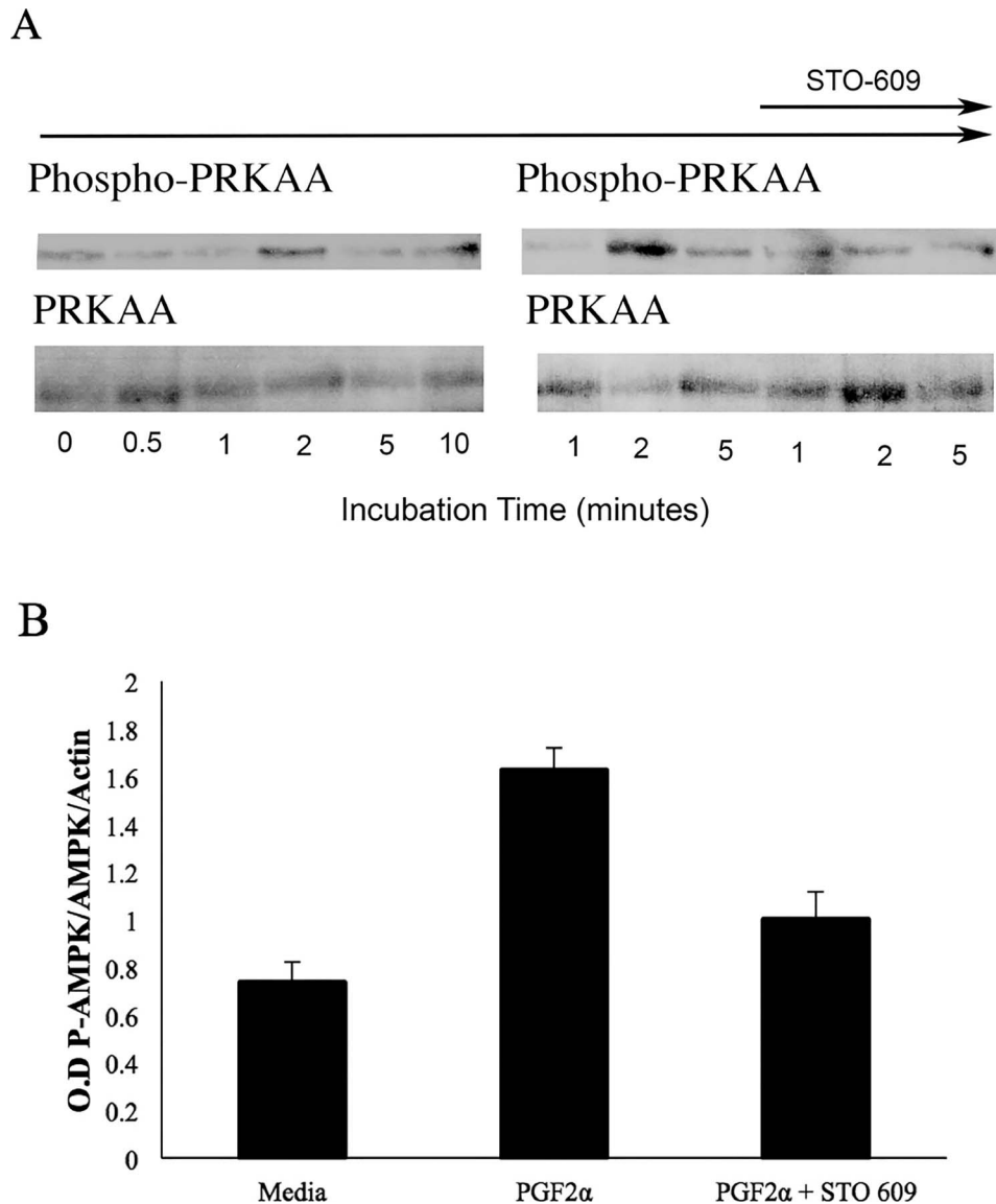
FIG. 2. Ability of PGF _{2\alpha} to activate PRKAA in steroidogenic luteal cells isolated from mature bovine CL. A ) Activation of FP induced rapid phosphorylation of PRKAA, and the CAMKK2 inhibitor, STO-609, abrogated this effect of PGF _{2\alpha} on AMPK ( P < 0.05 , indicated by different letters in B ). B ) Cells were treated with media alone, PGF _{2\alpha} (1.0 \mu g/ml) alone, or PGF _{2\alpha} and STO-609 (100 ng/ml) for 1, 2, or 5 min. Samples of isolated proteins were analyzed via Western blotting by probing the blots with specific antibodies for P-PRKAA, PRKAA, and actin proteins. Relative quantification was calculated after normalization of optical density (o.d.) determined for P-PRKAA normalized to its corresponding AMPK and then subsequently to actin. The y-axis shows the mean \pm SEM of the normalized o.d. determined for P-PRKAA divided by PRKAA and beta actin.
