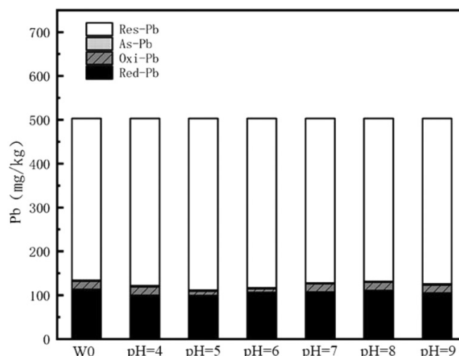
Fig. 8. Contamination soil group with 25 days passivation.
