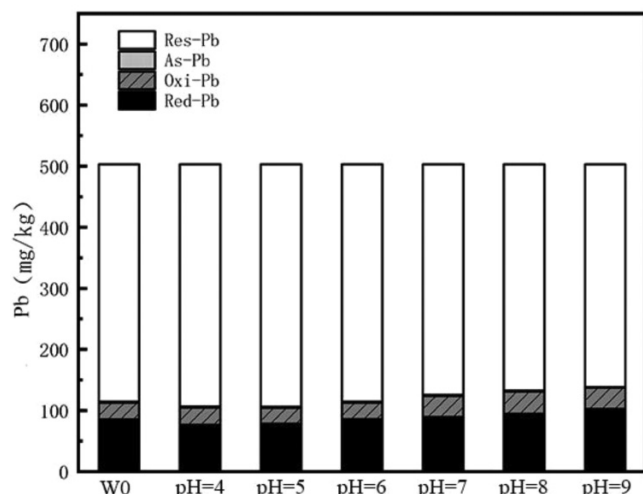
Fig. 7. Contamination soil group with 15 days passivation.
