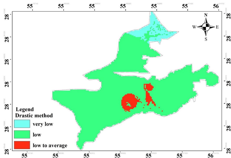
Figure 6. The vulnerability map of the DRASTIC model and the EC value in observation wells.
