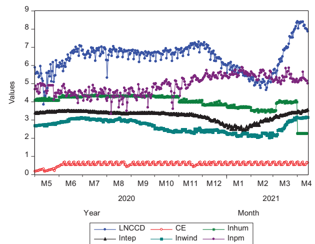
Figure 2. COVID-19 daily-confirmed cases versus climatic factors.
