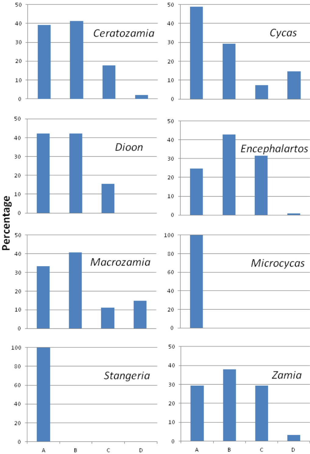
Appendix 4. The percentage of species within each listing Criterion grouped by the genera that contain threatened species. Direct count frequency distributions significantly differed among the genera ( P < 0.0001 , 386 total entries). A = reduction in population size. B = limited geographic range. C = small population size combined with reduction in population. D = highly limited population size.
