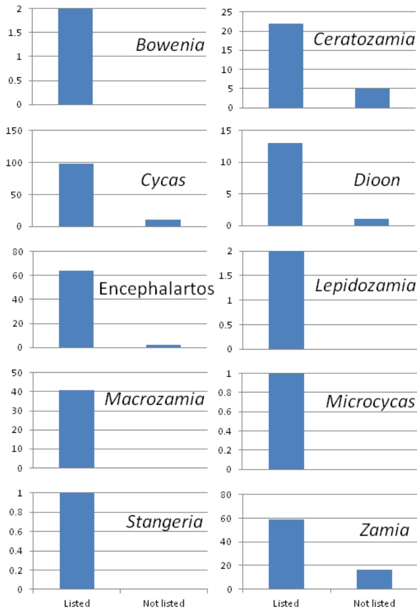
Appendix 5. Direct counts of species uploaded to the Red List or not found on the Red List for each of ten genera. Frequency distributions significantly differed among the genera ( P=0.0099 , 337 total entries).
