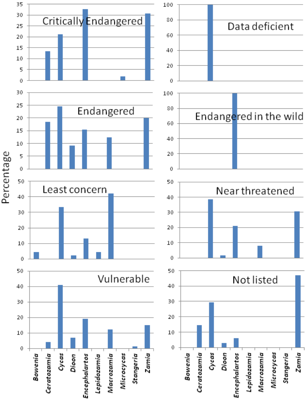
Appendix 1. The percentage of species among genera for each of seven Red List threat categories and the percentage of described species for each genus that are not contained on the Red List. Direct count frequency distributions significantly differed among the Categories ( P < 0.0001 , 337 total entries).
