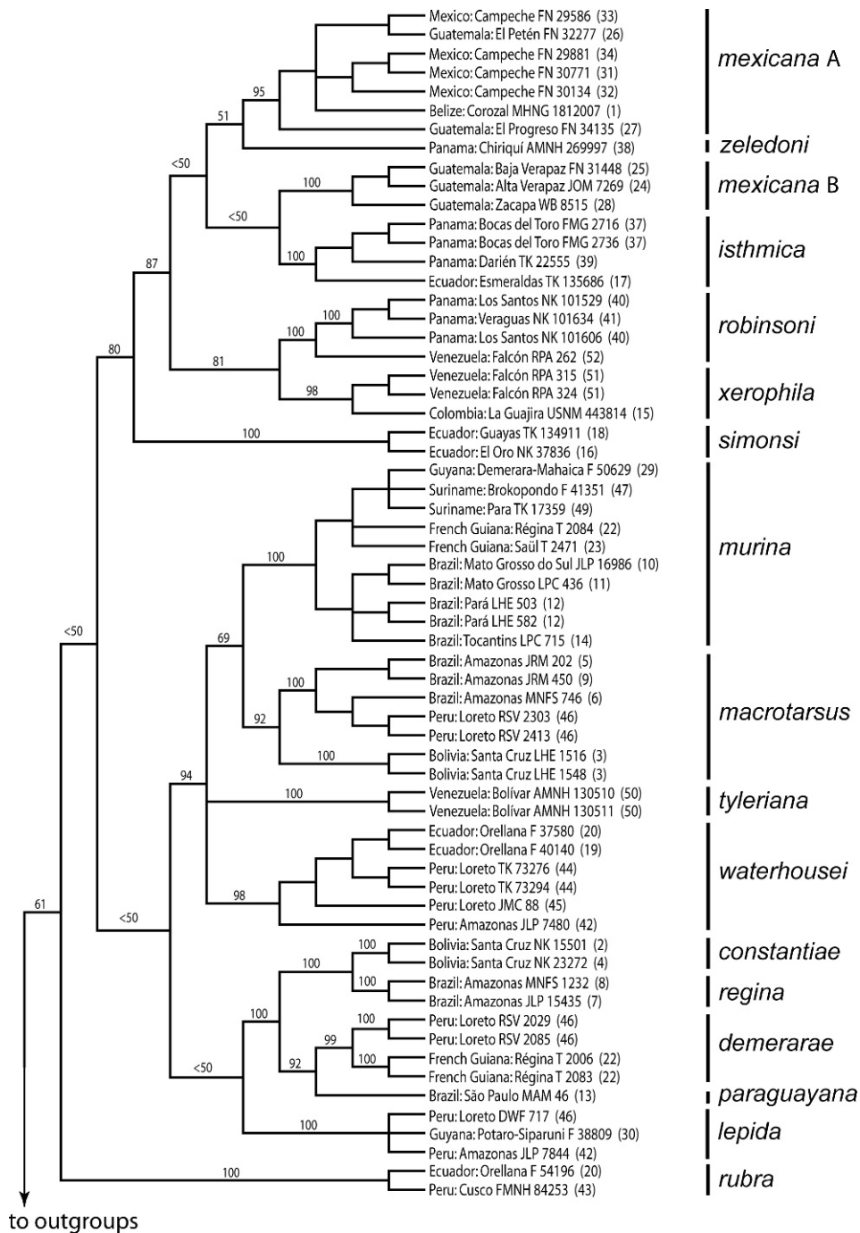
Fig. 2. Strict consensus of 96 equally most-parsimonious trees (L = 2198; CI = 0.36; RI = 0.80). Bootstrap support values are indicated above branches subtending species and conspecific haplogroups discussed in the text. For each terminal, country of origin, next-largest political unit (state, department, province, etc.), and an alphanumeric specimen identifier (from table 2) are provided. Numbers in parentheses refer to localities mapped in figure 1 and listed in the Gazetteer (appendix).
