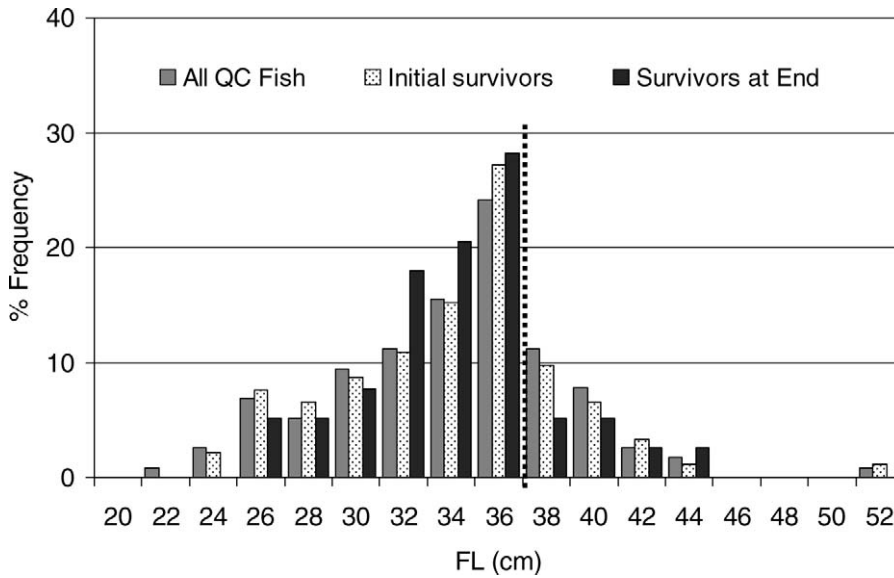
FIGURE 2.—Length frequencies (fork length [FL]) of red snapper: all quasicontrol (QC) fish captured (gray bars), survivors of immediate mortality (patterned bars), and survivors of delayed mortality (black bars). The dashed line represents the legal size limit of 37.7 cm FL (40.6 cm total length).
