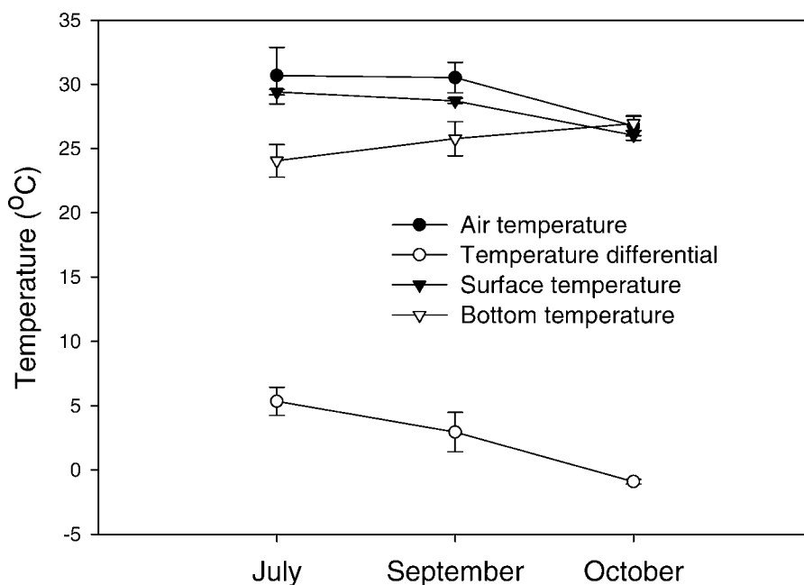
FIGURE 1.—Average ( \pm SD) monthly air temperatures measured in the shade where red snapper were measured on deck. Surface and bottom water temperatures were measured with a Sea-Bird SBE 19 conductivity–temperature–depth profiler. July and September air temperatures were significantly different from October air temperatures, while surface and bottom water temperatures and the temperature differential between surface and bottom waters differed significantly each month.
