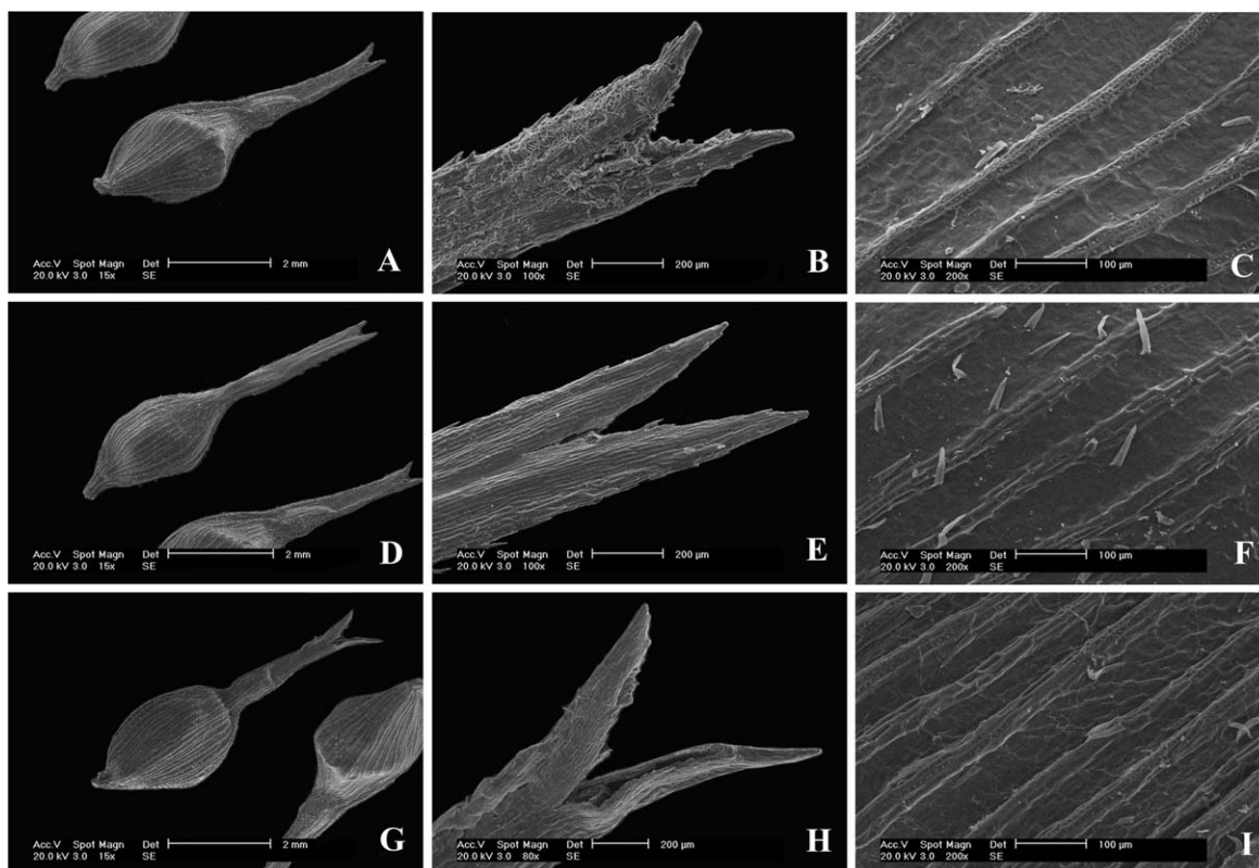
FIG. 3. SEM photographs of perigynia. A-C. Carex paracheniana . D-F. C. cheniana . G-I. C. brevicuspis . A, D, G. Whole view of perigymia. B, E, H. Short teeth of perigynia. C, F, I. Sculpture and indumentum of perigynium bodies.
