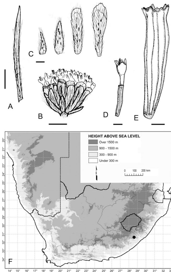
FIG. 14. Phymaspermum peglerae . A. Leaf. B. Capitula. C. Involucral bracts (outermost to innermost series, from left) and single palea (far right). D. Disc floret. E. Cypsela. F. Known geographical distribution. Voucher: A–E. Pegler 1601 (BOL). Scale: A–B = 4 mm; C–D = 1 mm; E = 500 \mu m.
