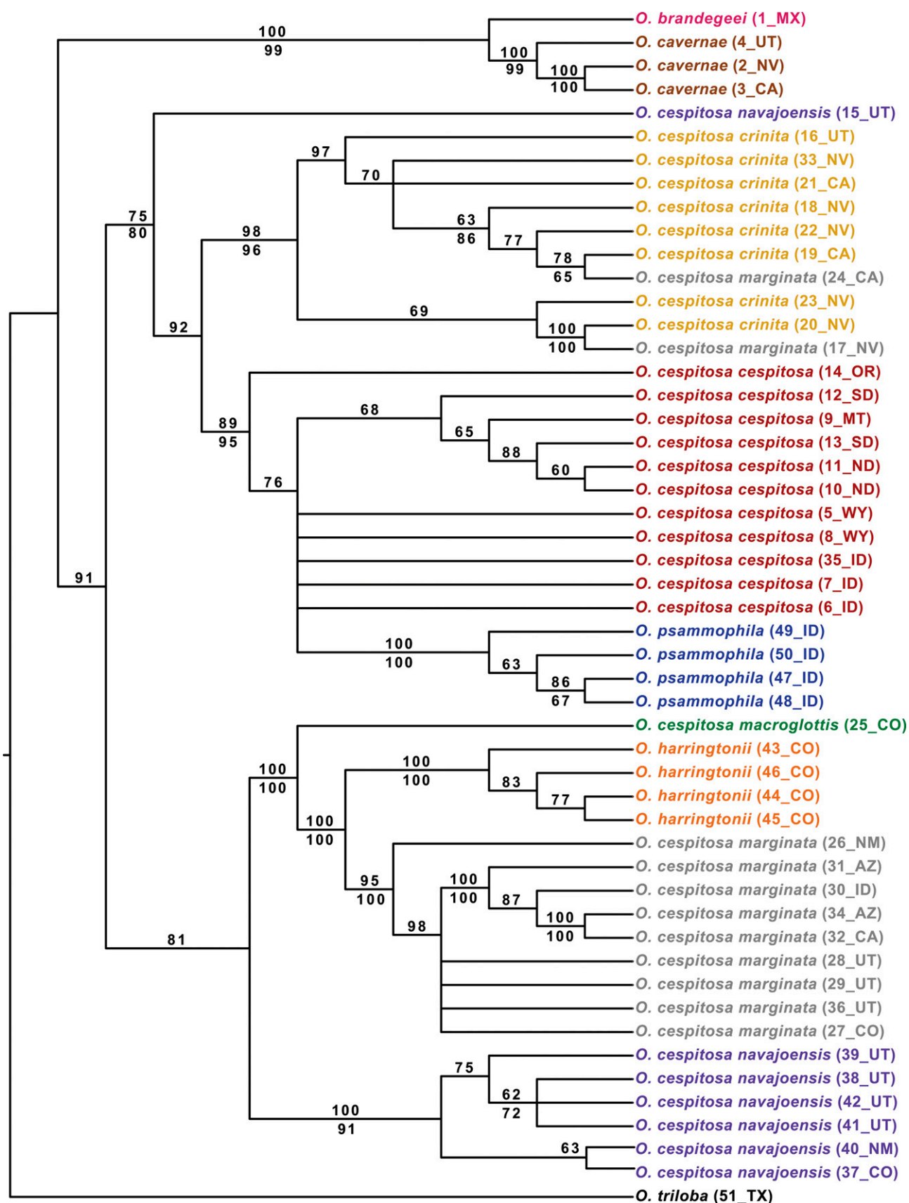
FIG. 4. Coalescent-based ASTRAL multilocus bootstrap consensus topology of Oenothera sect. Pachylophus inferred from 307 loci. Branches with multilocus bootstrap values < 60 are collapsed. Bootstrap values > 60 are shown; above the branches are the ASTRAL multilocus bootstrap values, and below the branches are the SVDquartets bootstrap values. Samples are colored by taxon, and an individual identifier (unique number and US state where the material was collected; see Appendix 1) is in parentheses following the taxon name.
