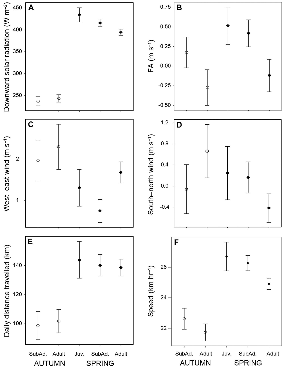
FIGURE 3. Mean ( \pm 95\% CI) for meteorological variables associated with daily migration of and for distances traveled by Golden Eagles in eastern North America, 2008–2015. Plots show (A) downward solar radiation, (B) flow assistance, (C) west–east surface wind vector, (D) south–north surface wind vector, (E) daily distance traveled, (F) hourly distance traveled. Autumn migration is represented by open circles and spring migration by filled circles. Sample sizes are in Appendix Table 5. Age classes of eagles are Juvenile (Juv.), sub-adult (SubAd.), and Adult; for details see Methods.
