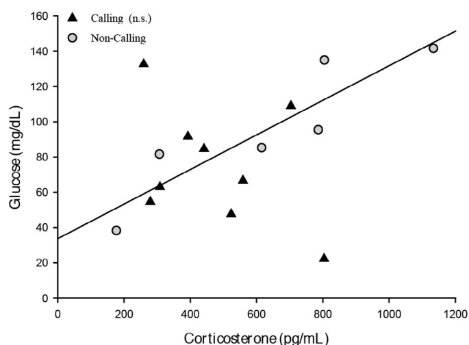
Fig. 7. Linear regression of circulating CORT and glucose concentrations in calling and non-calling males shows the amount of glucose in circulation positively correlates with circulating CORT within non-calling males ( R^2 = 0.665 ; \hat{Y}_i = 31.447 + 0.098X_i ; P < 0.001 ). The regression line is only indicative of a relationship between CORT and glucose concentrations for non-calling males, as there was no significant relationship between CORT and glucose in calling males ( R^2 = 0.149 ; P = 0.305 ).
