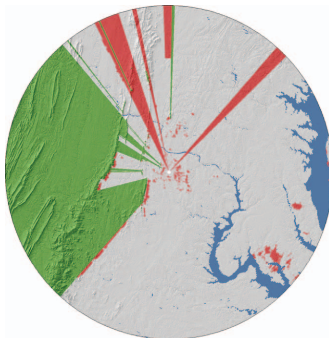
FIGURE 2. Masking map of the KLWX radar in Sterling, VA, showing sample volumes excluded from analyses due to (1) topographic beam blockage (green), (2) dominance of open water (blue), or (3) persistent ground clutter contamination and other sources of beam blockage (red).
