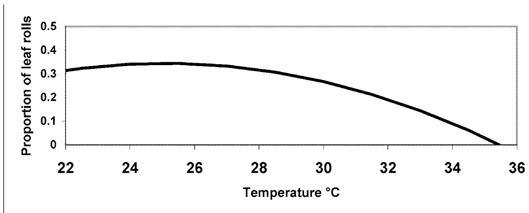
Fig. 2. Estimated effect of mean maximum temperature on proportion unfested subpinnae and mite induced leaf rolls (within sites). A higher proportion indicates a higher level of plant damage.
