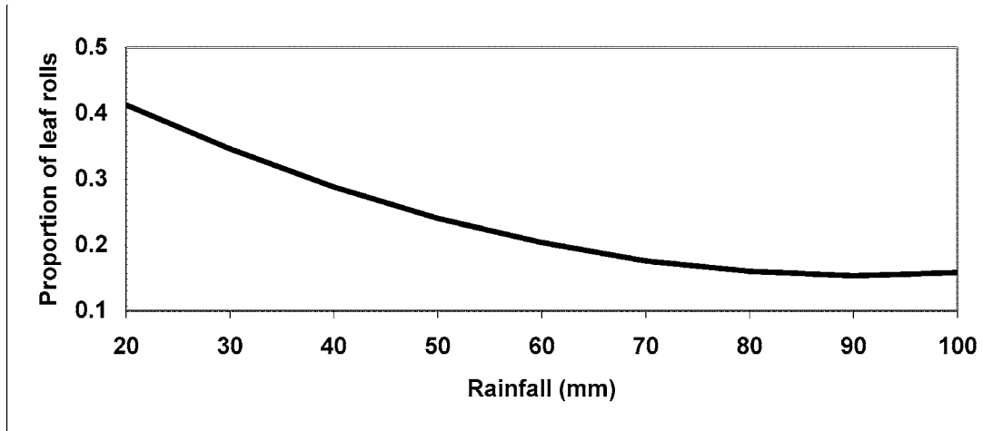
Fig. 1. Estimated effect of rainfall on annual proportion of unfested subpinnae and mite induced leaf rolls (between sites). A higher proportion indicates a higher level of plant damage.
