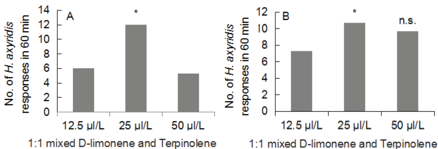
Fig. 8. Response of Harmonia axyridis adults to 12.5 \mu\text{L/L} , 25 \mu\text{L/L} , and 50 \mu\text{L/L} 1:1 mixed D-limonene and terpinolene after 60 min. A: No aphids; B: aphids present. The numbers of asterisks represent the level of significance: ** highly significant ( P < 0.01 ); * significant ( P < 0.05 ); n.s. no significant difference.
