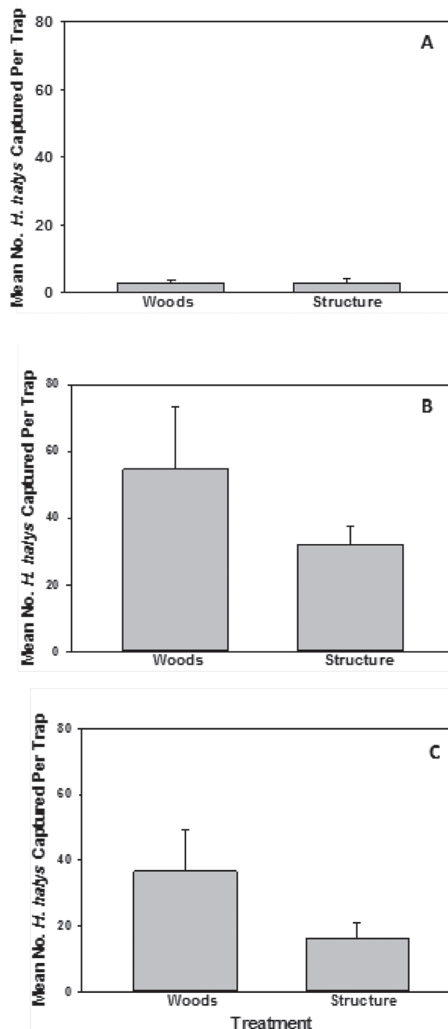
Fig. 2. Mean capture rates of Halyomorpha halys in black pyramid traps with fluorescent blue lights placed next to structures with competing light sources or next to wood line without competing lights, during early season (A), mid-season (B), and late season (C).
