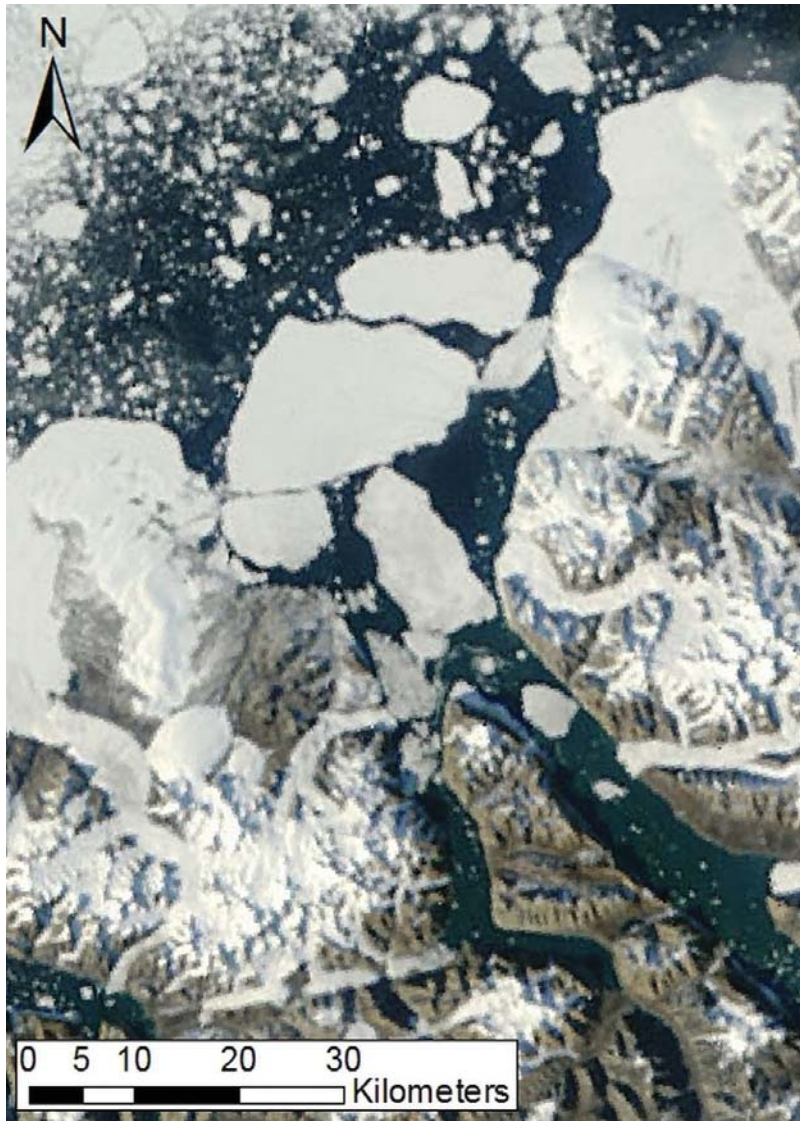
FIGURE 6. MODIS TERRA image (22 August 2010, 22:05 UTC) showing open water and floating ice in Yelverton Bay and Yelverton Inlet.
