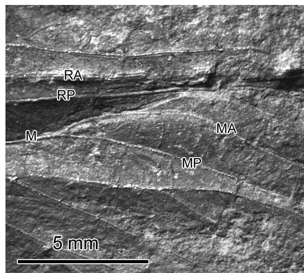
Fig. 3. Lobeatta schneideri gen. and sp. nov. (holotype specimen ROM 45568): detail of the area between RP and MP, photograph (right forewing, positive imprint, composite).
