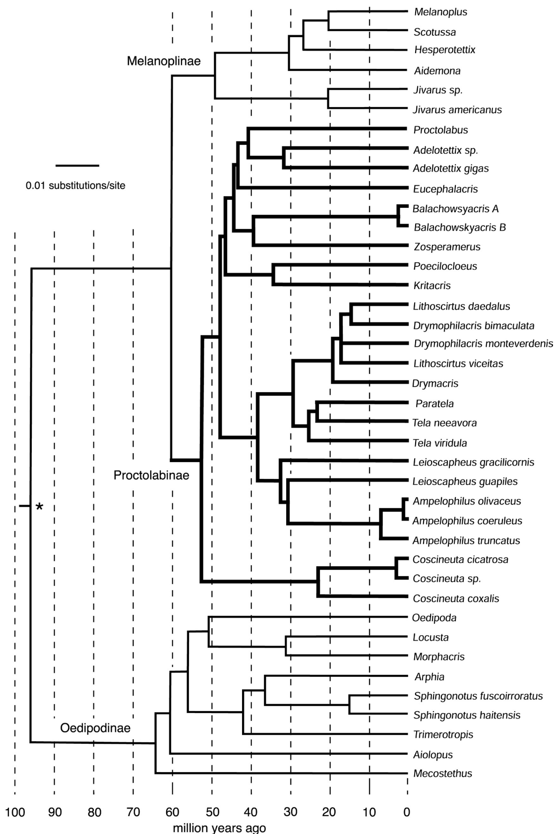
Fig. 4. Estimated timing of the evolution of the Proctolabinae, Melanopliinae and Oedipodinae. The tree is the strict consensus of 3 ultrametric ML trees with a molecular clock constraint; the calibration is based on the divergence (asterisked) of the Oedipodinae and remaining subfamilies at 97 Mya (Gaunt & Miles 2002). Further explanation in the text.
