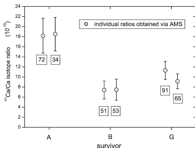
FIG. 3. Results of ^{41}\text{Ca}/\text{Ca} AMS measurements obtained from survivors who donated two teeth. The numbers in the boxes represent the sample-ID numbers in Table 5.
