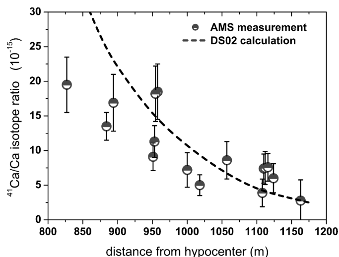
FIG. 4. Decrease of ^{41}\text{Ca}/\text{Ca} ratios with distance from the hypocenter. For comparison, DS02 calculations (dashed line) are shown, which were calculated without taking individual shielding conditions into account (free-in-air kerma dose, 1 m above ground; see Table 1). The error bars include all sources of uncertainties. A detailed comparison between measured and calculated ^{41}\text{Ca}/\text{Ca} ratios including the individual shielding situation of the survivors is given in ref. (51).
