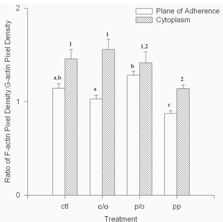
Figure 7. F:G-actin ratio in Heliothis virescens hemocytes. The ratio was determined by comparison of mean density of FITC-phalloidin staining to DNase I-rhodamine staining on a per cell basis at two focal distances in four treatment groups (see Fig. 6). Error bars are standard error of the mean, and different letters (z) and numbers (z+2.5μm) indicate means significantly differ at that focal distance at \alpha=0.05 .
