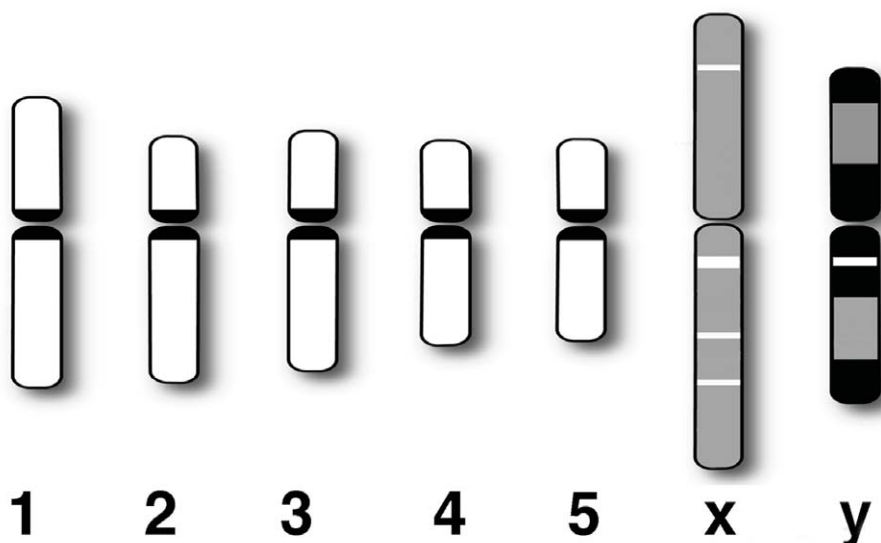
Figure 5. Diagrammatic representation of the C-banding idiogram of a male Scathophaga stercoraria . Strongest labeling is depicted in black, weaker labeling in grey and C-banding negative regions are depicted in white. High quality figures are available online.
