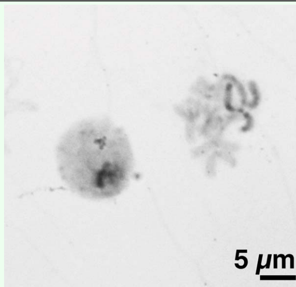
Figure 4. C-banding of a representative mitotic cell spread of a male Scathophaga stercoraria . Both sex chromosomes are more darkly stained than the C-band negative regions of the autosomes, and the Y chromosome additionally exhibits extensive darkly stained blocks. The autosomes are C-banding negative except for narrow bands in the centromeric regions. High quality figures are available online.
