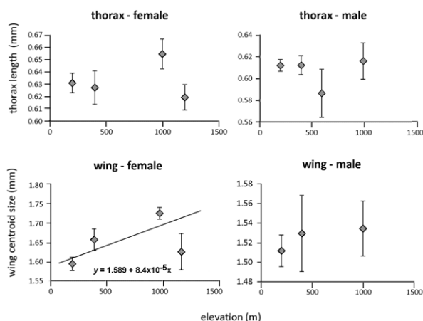
Figure 3. Thorax length and wing centroid size of female and male Liriomyza sativae at different elevations. Values are means \pm standard errors values. Linear regression lines and equation predicting size (y) from elevation (x) are shown on one graph where a significant association was detected. High quality figures are available online.
