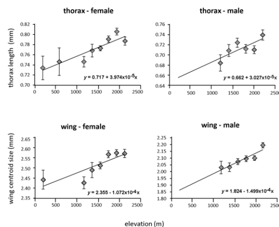
Figure 2. Thorax length and wing centroid size of female and male Liriomyza huidobrensis plotted against elevation. Values are means \pm standard errors. Linear regression lines and equations predicting size (y) from elevation (x) are shown on the graphs. High quality figures are available online
