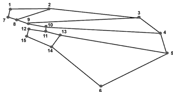
Figure 1. Positions of 15 landmarks on the wing of females and males of L. huidobrensis and L. sativae used for wing measurements. High quality figures are available online
