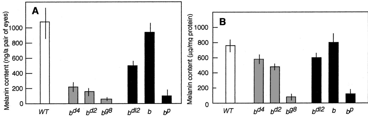
Fig. 3. Melanin content of the mutant eyes. (A) Fry, (B) Adult. b d4 and b d2 , ENU-induced; b g8 , γ-ray-induced (gray column); b dl2 , b , and b p , spontaneous (black column).
