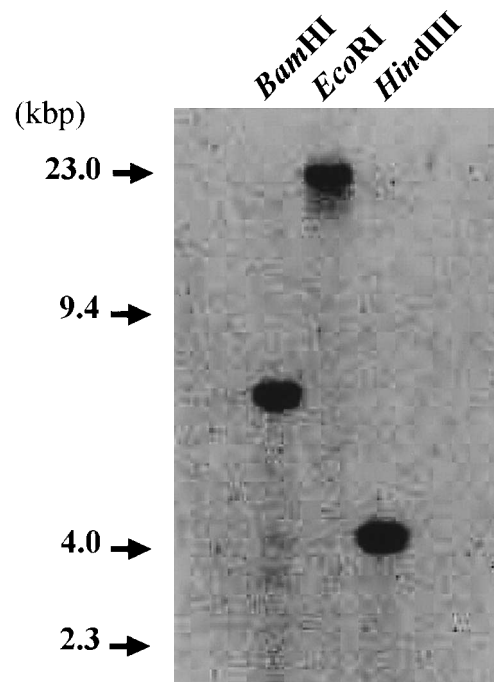
Fig. 6. Genomic Southern hybridization analysis. Genomic DNA (10 \mu g) from a single individual of the O. latipes Hd-rR inbred strain was digested with Bam HI, Eco RI, or Hind III. The blot was hybridized with a ^{32} P-labeled OIGC8 cDNA probe.
