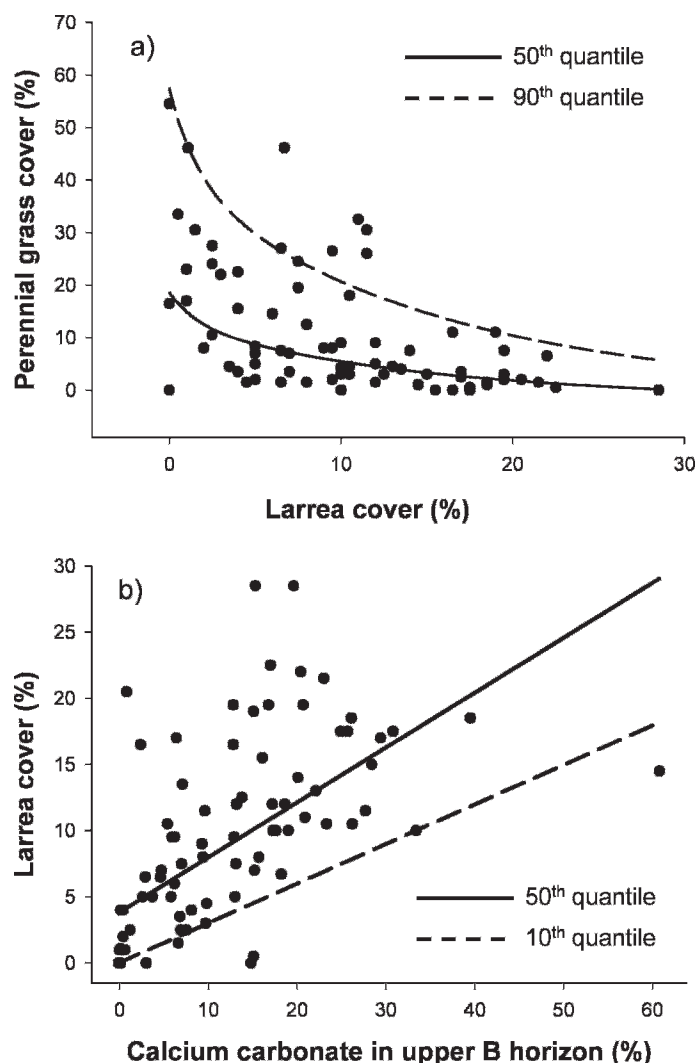
Figure 3. a , Relationship between percent canopy cover of Larrea tridentata and perennial grass cover in the valley border ballena soil-geomorphic system. The solid line is fit to a negative binomial function for the 50th quantile and the dashed line to the 90th quantile. See text. b , Relationship between percent calcium carbonate in the shallowest B soil horizon (e.g., Btk1) and percent canopy cover of Larrea tridentata . The solid line is fit to a linear function for the 50th quantile and the dashed line to the 10th quantile.
