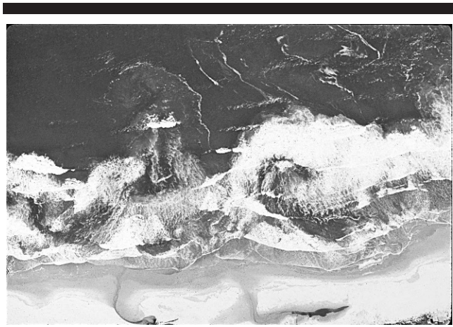
Figure 5. Massive rip currents occur at Ocean Beach, San Francisco, California, where the beach is always posted for no swimming, yet many drownings have been recorded. The rip current is nearly impossible to detect by beachgoers at ground level, but is apparent from this aerial view (photo by Dr. Stephen P. Leatherman).
