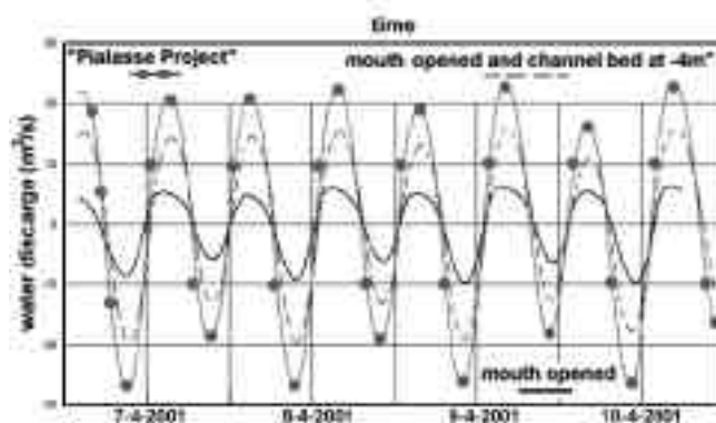
Figure 6. Water discharge variations of Bellocchio channel under three different scenarios: channel mouth opened only, channel mouth opened and bed excavation to -4 meters and transformation of Bellocchio salt marshes in "Piailasse".
