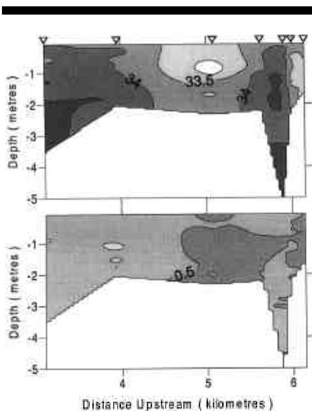
Figure 6. Saltwater Creek at high tide showing a) salinity structure with a contour interval of 0.5 ppt and b) light transmission with a contour interval of 0.05 uncalibrated transmission units. Data were collected on 26/09/2001 at 1730 hrs which corresponded to the high tide and maximum velocity levels presented in Figure 5.
