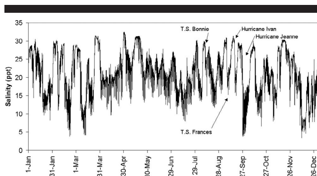
Figure 9. Salinity at Cat Point, 2004.
