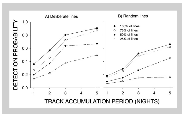
Figure 1. Estimates of the probability of detecting lynx for deliberate (A) and random (B) census strategies as a function of days (1-5) after snowfall. The different lines in the figure represent different densities of census lines with 100% representing 1 line/38 km 2 . Detection probability is mean of the detection probability for individual lynx. For each day after snowfall lynx was included in the computation if data were available for ≥ 5 periods.
