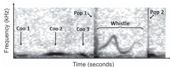
Figure 2. Example of a vocalization from a typical male greater sage-grouse Centrocercus urophasianus from a lek in Fremont County, Wyoming. This recording was captured using an on-lek microphone array (Krakauer et al. 2009) instead of the more distant single-microphone recording technique used in this study. This microphone set-up illustrates the full suite of vocal characteristics, some of which are not visible in the spectrograms produced by the microphone used in this study.
