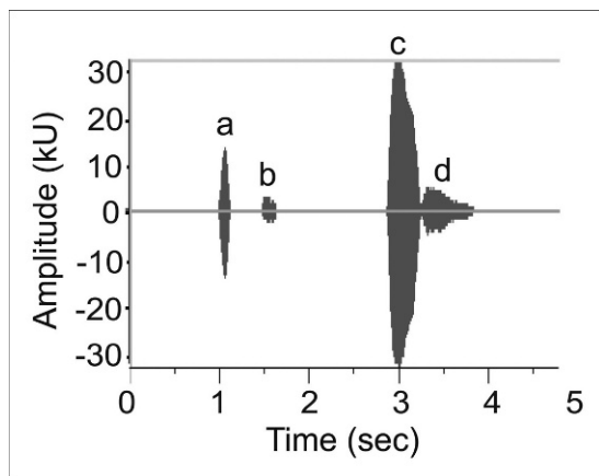
Figure 2. Oscillogram of Blakiston's Fish-Owl duet recorded May 2006 near Olga, Primorye, Russia. From left, male vocalizations are parts a,c; female vocalizations are parts b,d. Oscillogram generated using Raven 1.1 software (Cornell Bioacoustics program, Ithaca, NY, U.S.A.).
