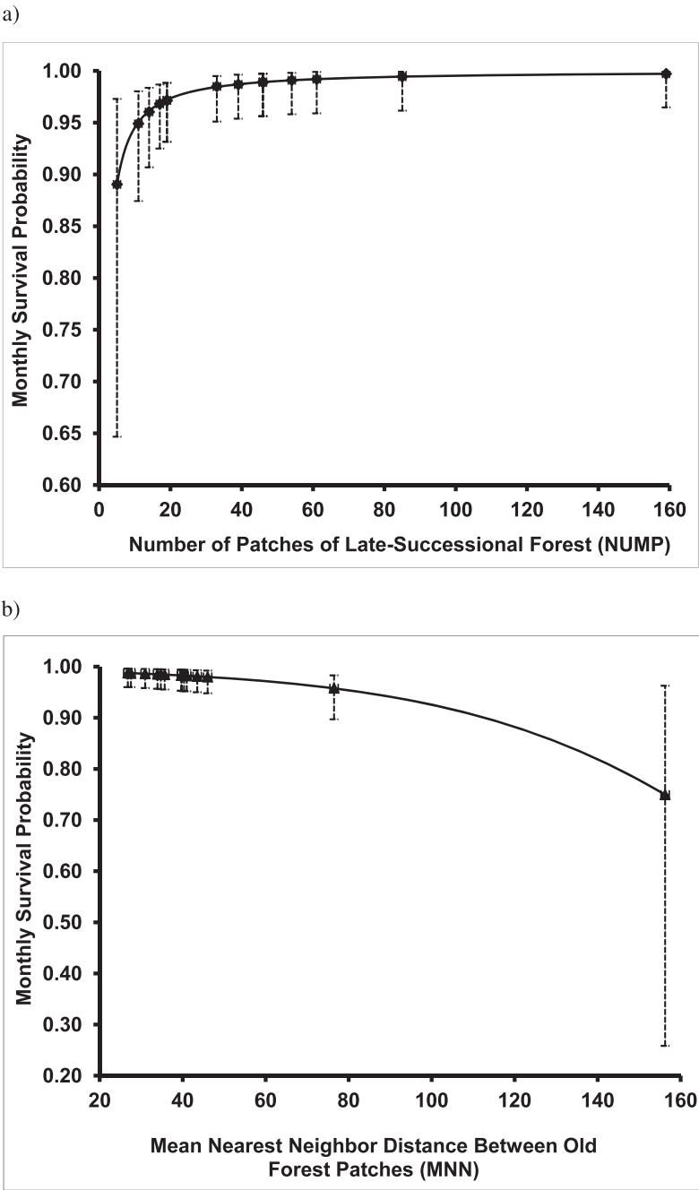
Figure 1. Monthly survival rates from (a) the best model, S_{(lg\_Nump)} plotted against the number of late-seral forest patches and (b) a competitive model S_{(MNN)} plotted against mean nearest neighbor distances (m) between late-seral forest patches within individual Northern Spotted Owl home ranges in southern Oregon, 2006–08.
