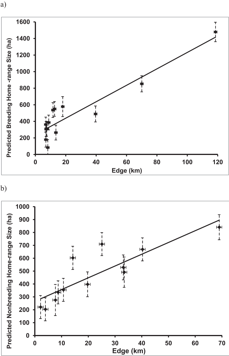
Figure 3. Home-range size estimates from the best model best model ( HR_{EDGE} ) plotted against the amount of edge (km) for (a) 13 Northern Spotted Owls during the breeding season and (b) 12 Northern Spotted Owls from the nonbreeding season during 2006–08 in the Siskiyou Mountains of Oregon.
