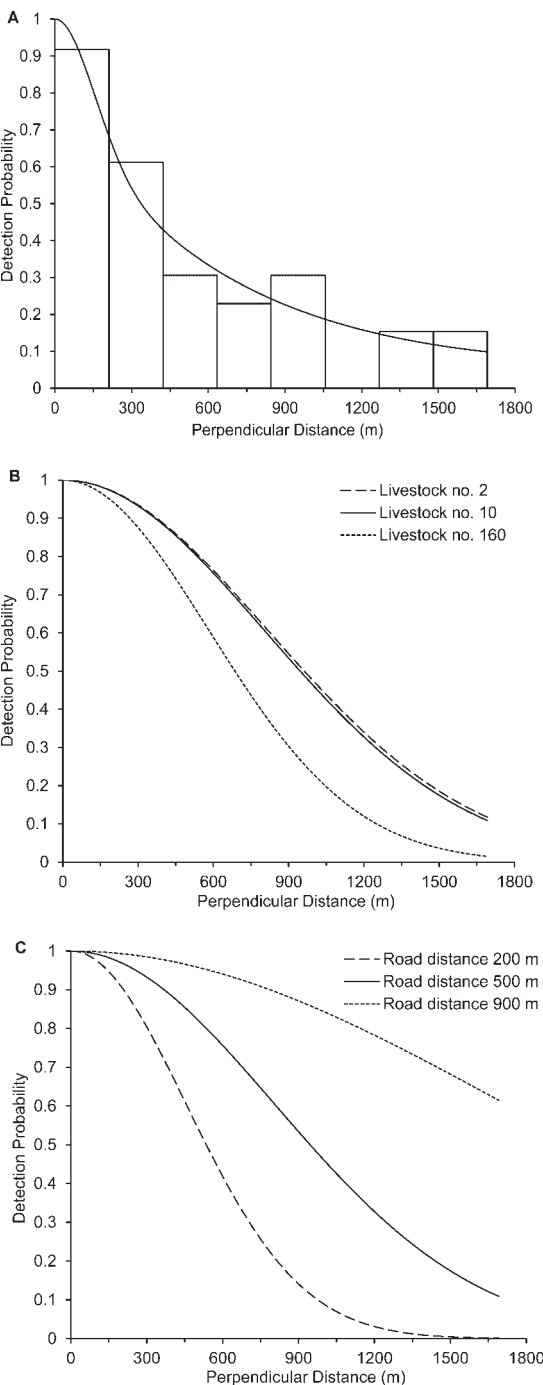
Figure 2. Histograms of detection of Bearded Vultures along line transects: (a) a half-normal detection function of Bearded Vultures from the line transects using the multiple covariate distance sampling (MCDS) engine with covariates livestock number and distance to road and fitted detection
