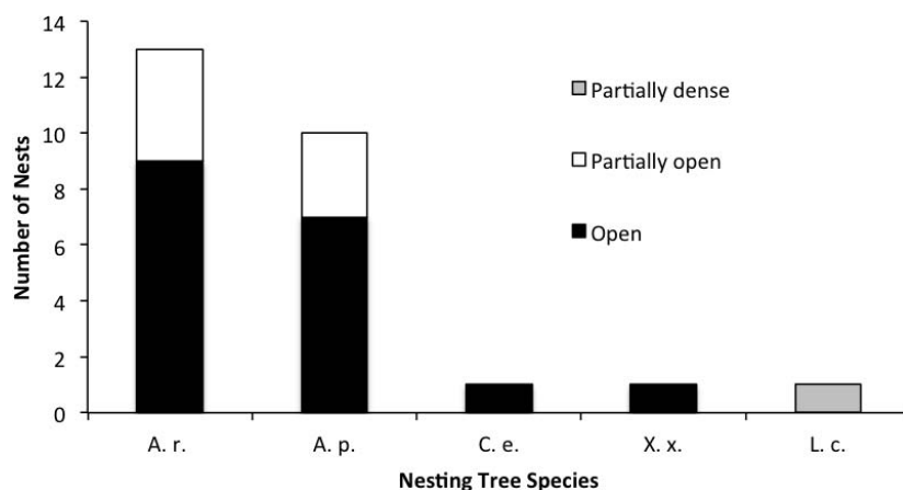
Figure 2. Crown density of nest trees of Grey-headed Fish-Eagles ( Ichthyophaga ichthyaetus ) at Noakhali, Bangladesh. Crown density is shown as three categories: Open: 0–25% canopy closure, Partially open: 26–50% canopy closure, and Partially dense: 51–75% canopy closure. A. r.: Albizia richardiana , A. p.: Albizia procera , C. e.: Casuarina equisetifolia , X. x.: Xylia xylocarpa , and L. c.: Lannea coromandelica .
