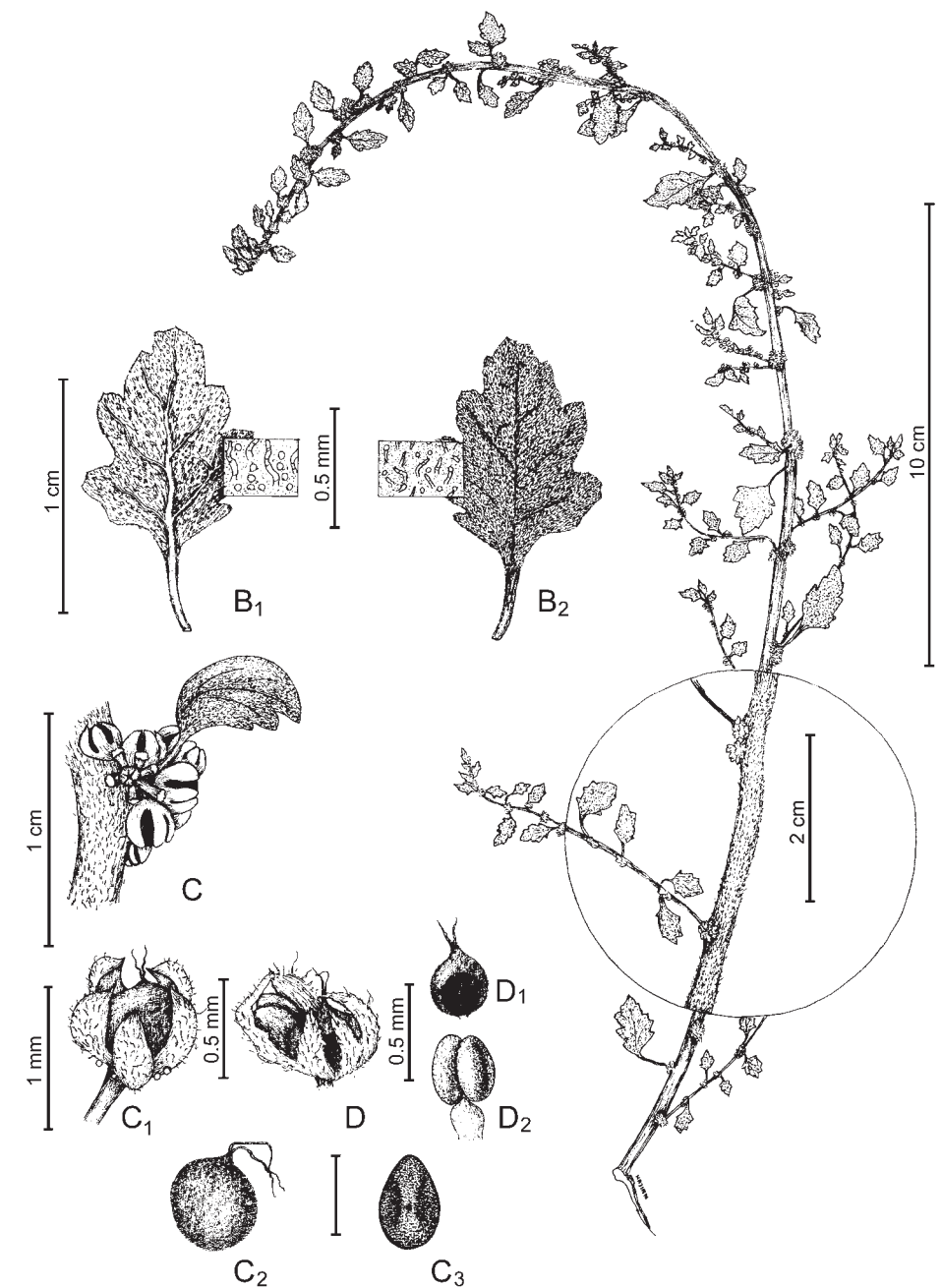
Fig. 1. Chenopodium pumilio – A: habit; B: leaf, (1) lower surface, (2) upper surface; C: compact axillary cyme with shortly pedunculate flowers, (1) female flower, (2) pistil, (3) seed; D: hermaphrodite flower, (1) pistil, (2) stamen.
