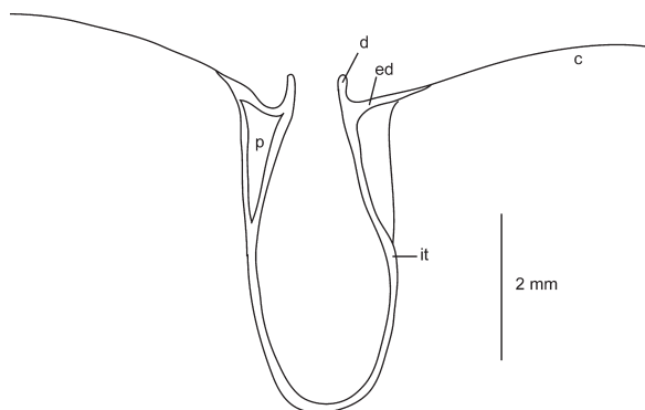
Fig. 3. Lomelosia solymica – half-schematic section of epicalyx. – c = corona, d = diaphragma, ed = epidialphragma, it = involucre tube, p = pits; initial pits (= foveoles) indicated by dotted lines.
