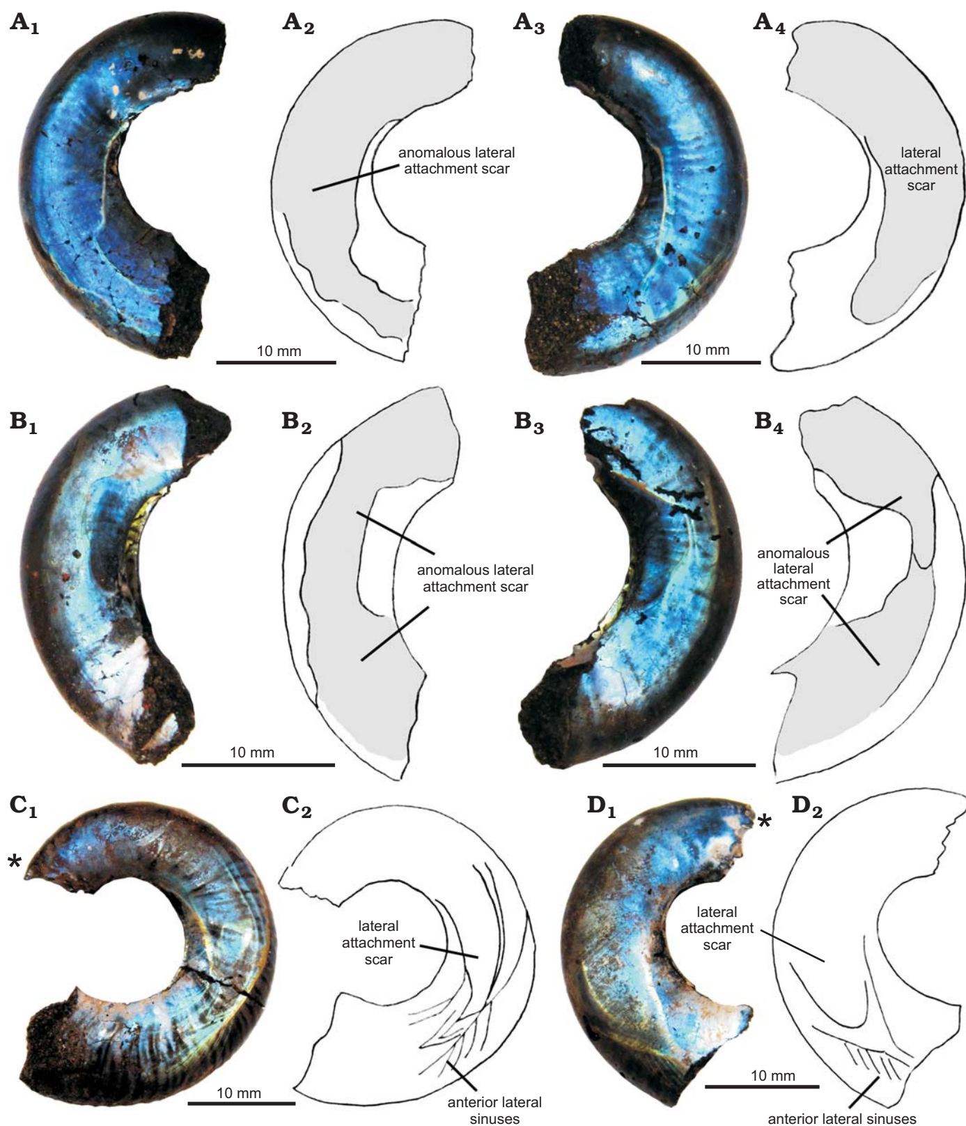
Fig. 8. Abnormal lateral attachment scars and lateral sinuses on Kachpurites fulgens (Trautschold, 1861) shells from Late Volgian ( Kachpurites fulgens Zone), Moscow region, Mnevniki locality. A. MSU 113/26, fragment of the body chamber with scars visible on both sides of the shell, normal shape scar (A 3 , A 4 ), anomalous scar-merged with anterior lateral sinuses (A 1 , A 2 ). B. MSU 113/25, fragment of the body chamber with anomalous scars merged with lateral sinuses on both sides of the shell. C. MSU 113/2, body chamber with abnormal scars merged with lateral sinuses. The apertural part is not preserved. D. MSU 113/16, posterior part of body chamber. Visible two growth stages of scars: a later-formed with a sharp-edged border and an earlier-formed rounded inside the first one. Asterisks mark the base of the body chamber. Photographs (A 1 , A 3 , B 1 , B 3 , C 1 , D 1 ) and explanatory drawings (A 2 , A 4 , B 2 , B 4 , C 2 , D 2 ).
