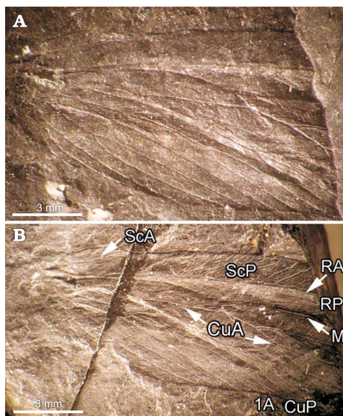
Fig. 7. Anthracoptilid insect Westphaloptilus gallicus sp. nov. from Bashkirian of Bruay-en-Artois, Department of North, France, holotype Bruay F.5 BR27–28, photograph of imprint (A), photograph of counterimprint (B). 1A, first anal vein; CuA/P, cubitus anterior/posterior; M, indistinguishable polarity of median vein; RA/P, radius anterior/posterior; ScA/P, subcosta anterior/posterior.
