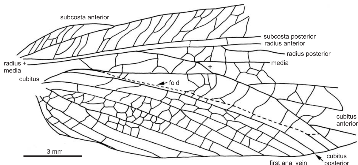
Fig. 6. Forewing of anthracoptilid insect Westphaloptilus gallicus sp. nov. from Westphalian of Bruay-en-Artois, Department of North, France, holotype Bruay F.5 BR27–28.
