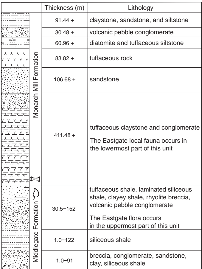
Fig. 2. Basic stratigraphic column of the Monarch Mill and Middlegate formations showing the dominant lithologies (modified from Axelrod 1956). The general stratigraphic positions of the Eastgate local fauna and flora are indicated with the appropriate symbols. The specific units dated by Stewart et al (1999) and Swisher (1992) are not shown because of the paucity of available data.
