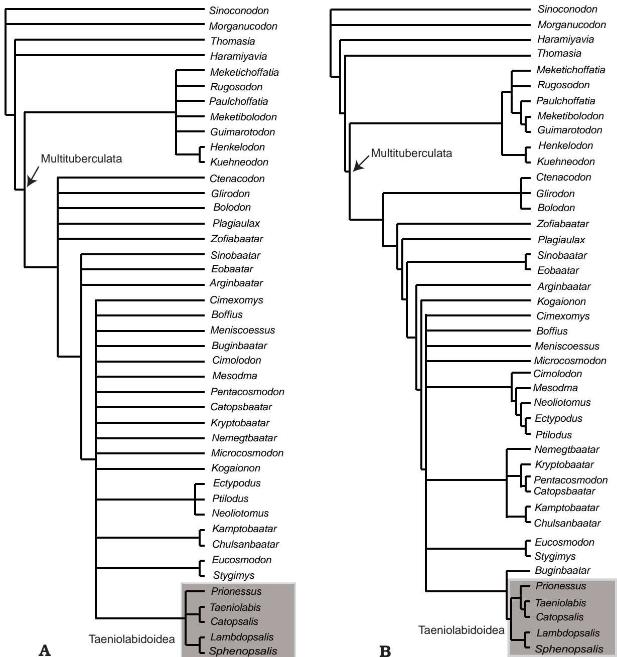
Fig. 17. Phylogenetic position of Sphenopsalis nobilis within multituberculates. A. The strict consensus tree of 138 trees obtained in the PAUP search where 19 characters were ordered (see SOM). B. The 50% majority rule consensus tree with 19 characters ordered. See additional supporting data in the SOM.
