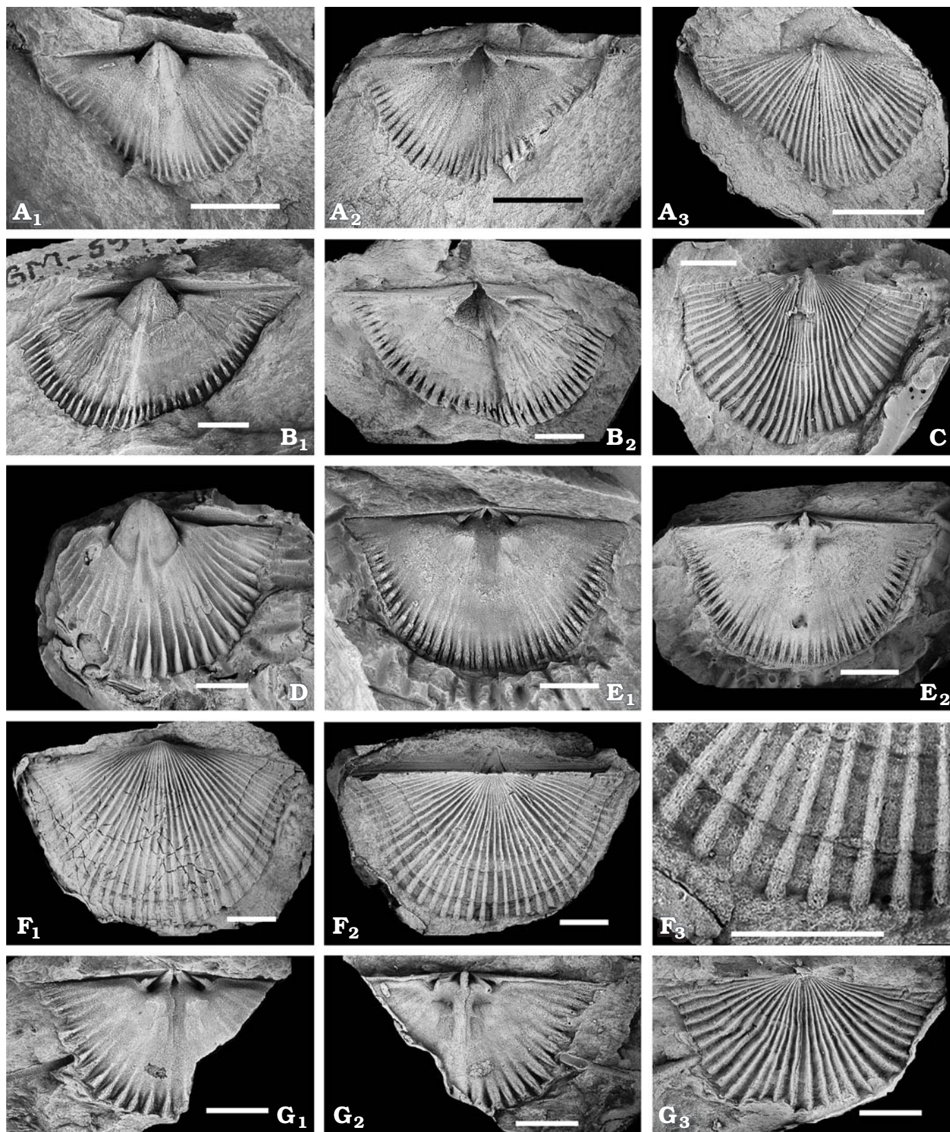
Fig. 6. Orthid brachiopod Paralenorthis alata (J. de C. Sowerby in Murchison, 1839). A. MGM-6021-O internal mould (A 1 ), latex cast of interior (A 2 ) and latex cast of exterior (A 3 ) of ventral valve. B. MGM-6030-O, internal mould (B 1 ) and latex cast of interior (B 2 ) of ventral valve. C. MGM-6038-O, latex cast of exterior of ventral valve. D. MGM-6037-O, internal mould of ventral valve. E. MGM-6048-O internal mould (E 1 ) and latex cast of interior (E 2 ) of dorsal valve. F. MGM-6027-O, latex cast of ventral exterior (F 1 ), latex cast of dorsal exterior (F 2 ), and detail of the latter (F 3 ) of a shell with conjoined valves. G. MGM-6042-O, internal mould (G 1 ), latex cast of interior (G 2 ) and latex cast of exterior (G 3 ) of dorsal valve. Scale bars 5 mm.
