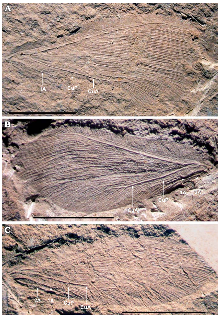
Fig. 2. Forewings of undescribed archeosmylid insects from the Madygen Formation, Middle to Upper Triassic, Kyrgyzstan, Central Asia. A. PIN 2785/4081. B. PIN 2555/ 2096. C. PIN 2069/3604. Scale bars 5 mm. Abbreviations: 1A, 2A, anal veins; CuA, anterior cubitus; CuP, posterior cubitus.
