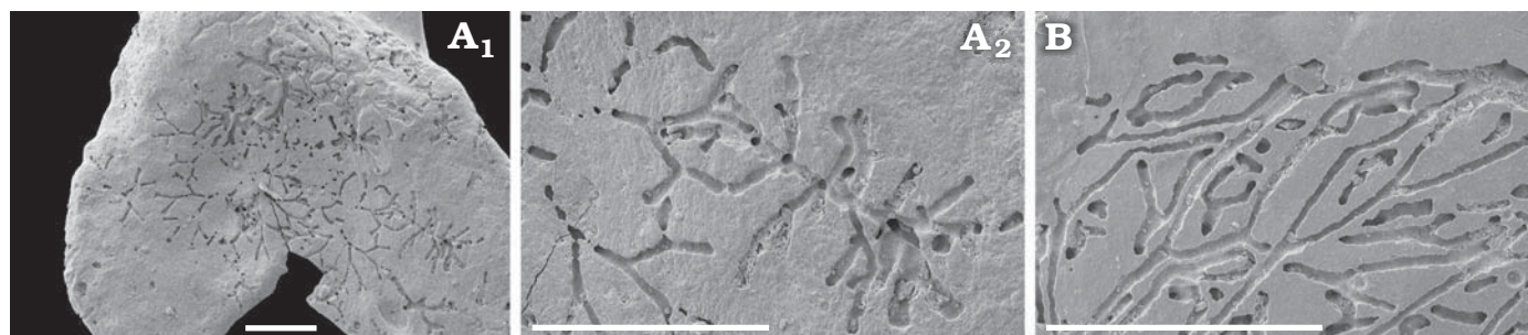
Fig. 3. Microborings in the Miocene shark teeth from Cerová section in Malé Karpaty, Slovakia. A. SNM Z 27430, bed 20–21. Two different sizes of Abeliella riccioiodes Mägdefrau, 1937 and an unnamed boring in a tooth root ( Squaliolus ) ( A 1 ). Detail of unnamed boring from A 1 ( A 2 ). B. SNM Z 27431, bed 8–9. Mycelites ossifragus Roux, 1887 at a tooth crown-root junction ( Paraetmopterus ). Scale bars 0.1 mm.
